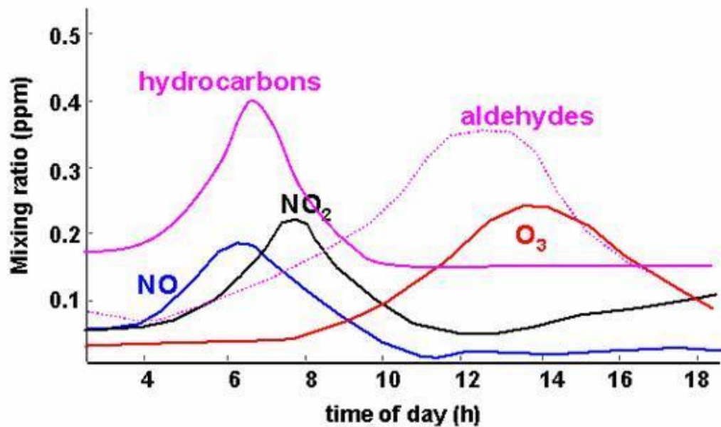
Typical evolution of a photochemical smog
