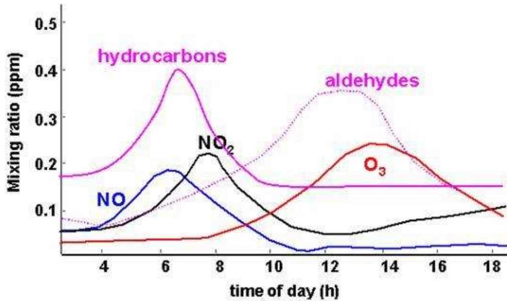
Typical evolution of a photochemical smog
